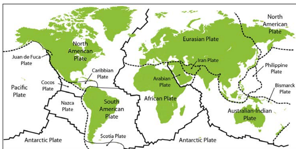
Figure 5.1 Lithosphere plates
